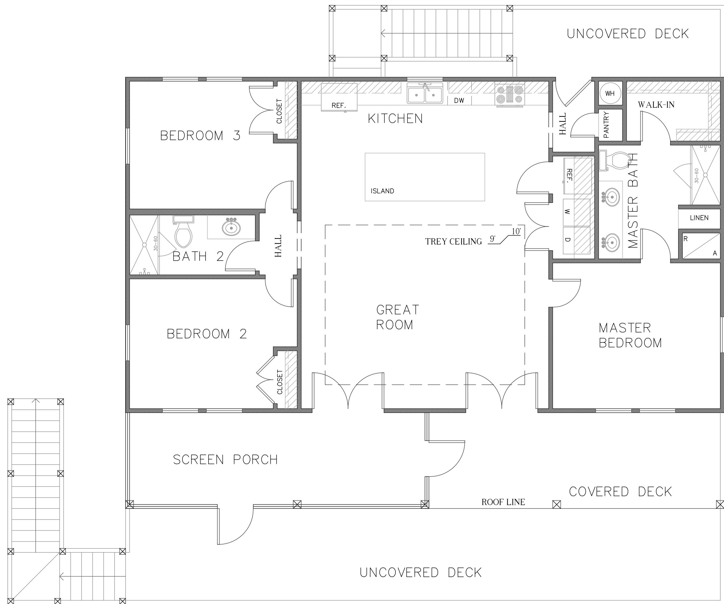
FLOOR PLAN
