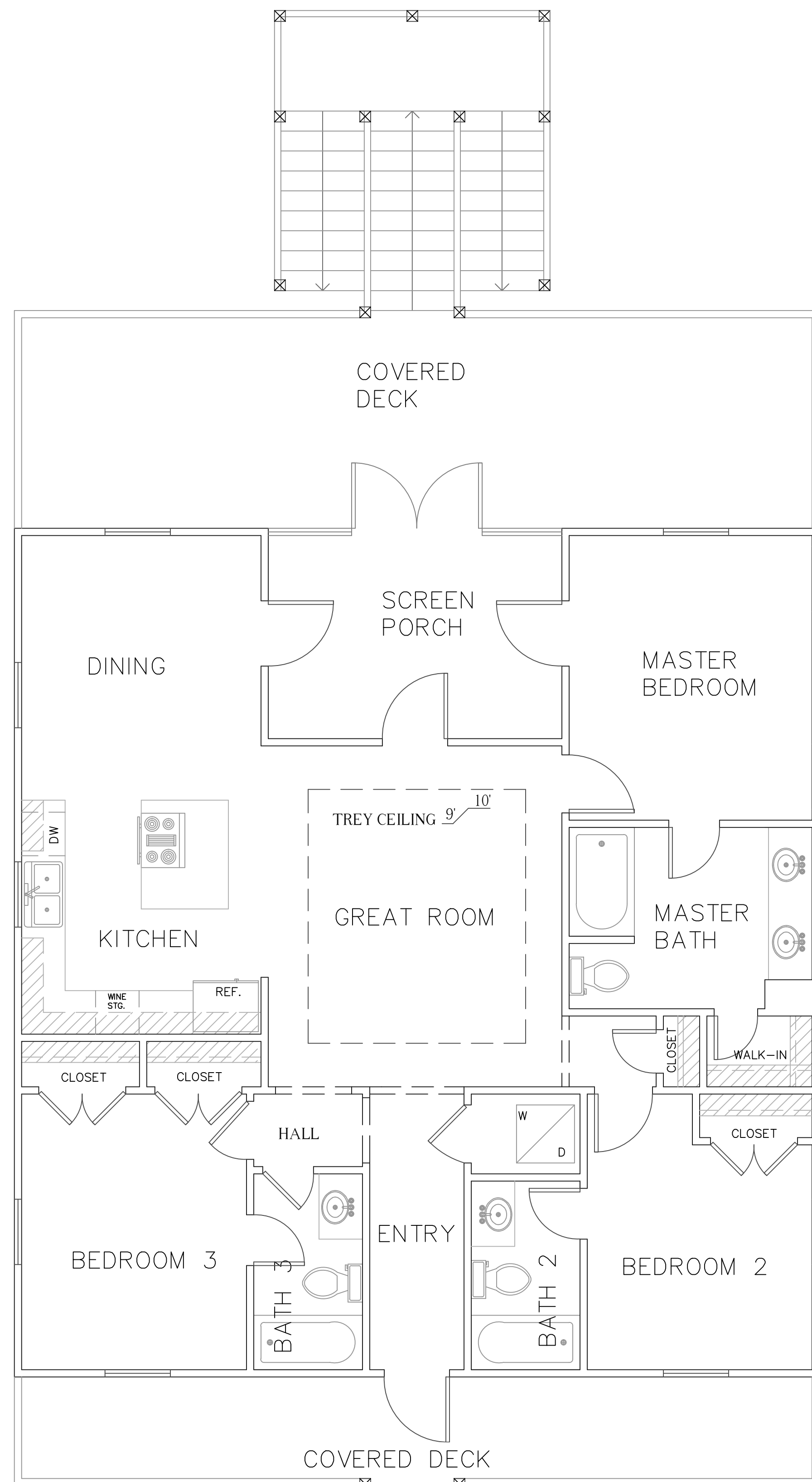
FLOOR PLAN
