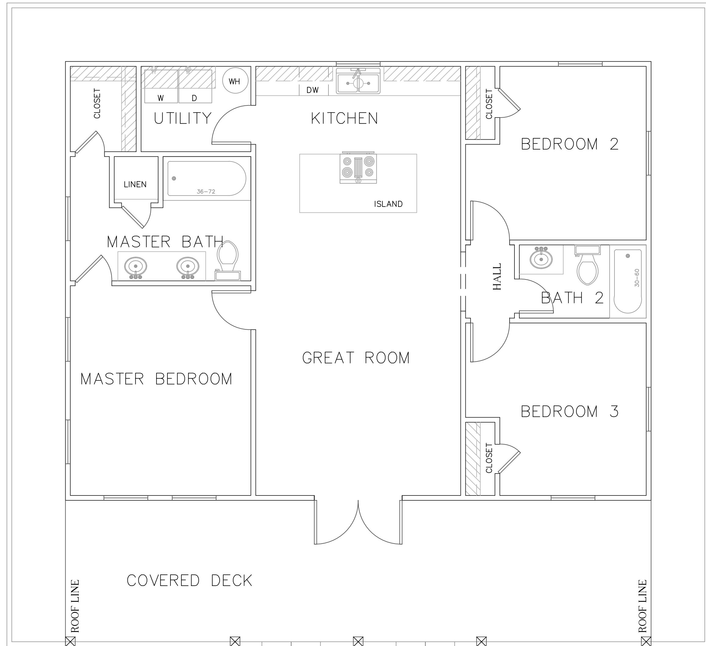
FLOOR PLAN
